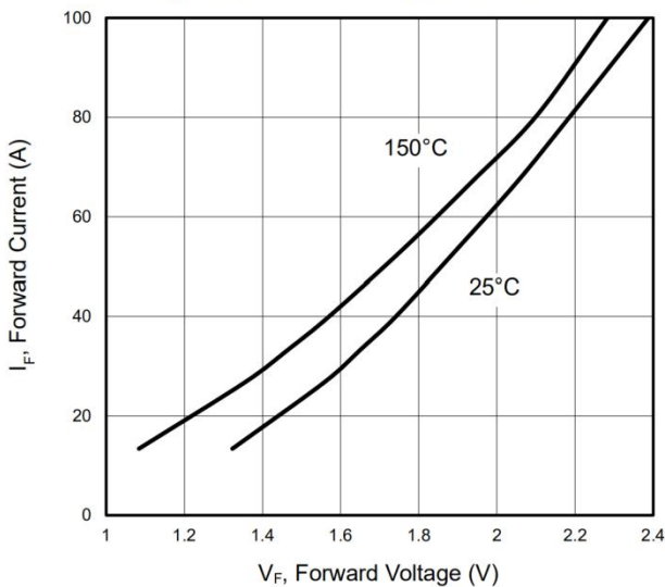
Figure 7 Forward Characteristics
